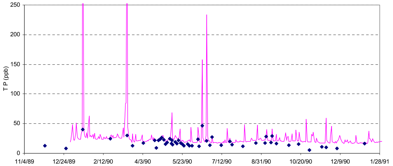
Figure 13. Simulated and observed total phosphorus at station 2, Platte River below hatchery
